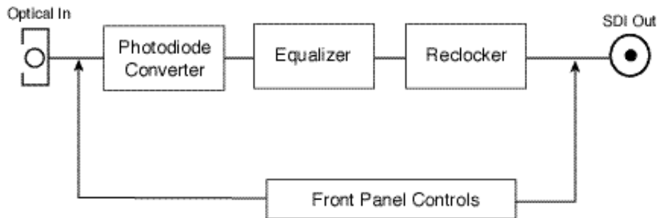
BrightEye 12 Functional Block Diagram
