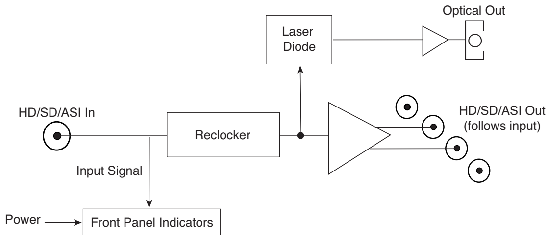
BrightEye 45 Functional Block Diagram
