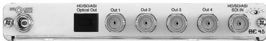
BrightEye 45 Rear Connectors
