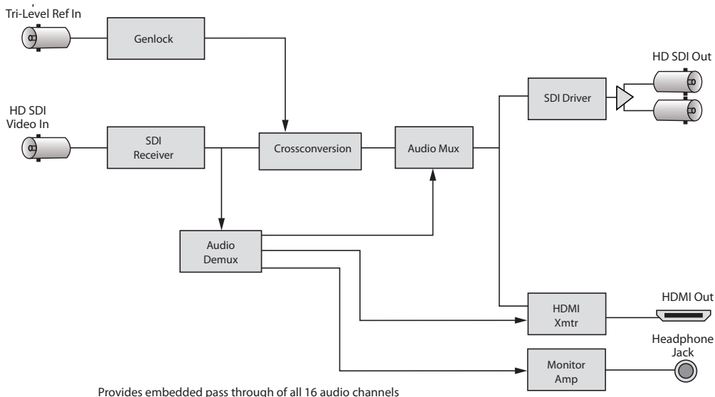
BrightEye 93 Functional Block Diagram, portrait view
