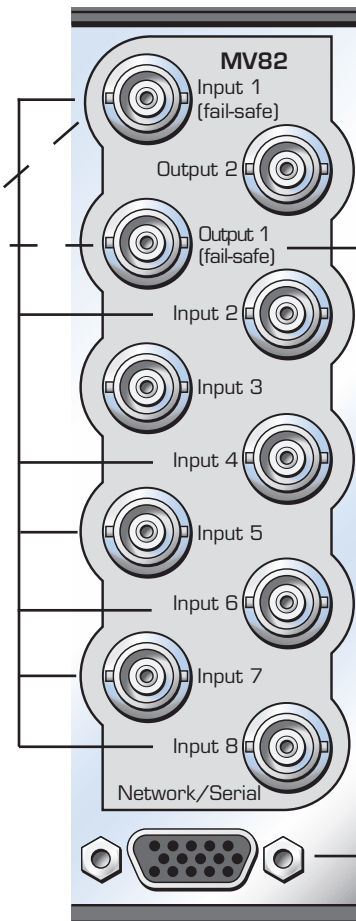
3RU Backplane
